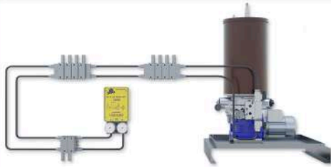
Dual Line System
