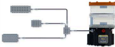
Single Line Progressive System
