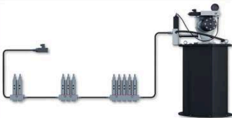
Single Line Unit Injector System
